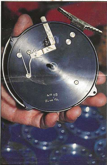
10. The centre bush bearing, the spokes, springs and other component parts are assembled with care and the backplate fitted with a ratchet mechanism.
